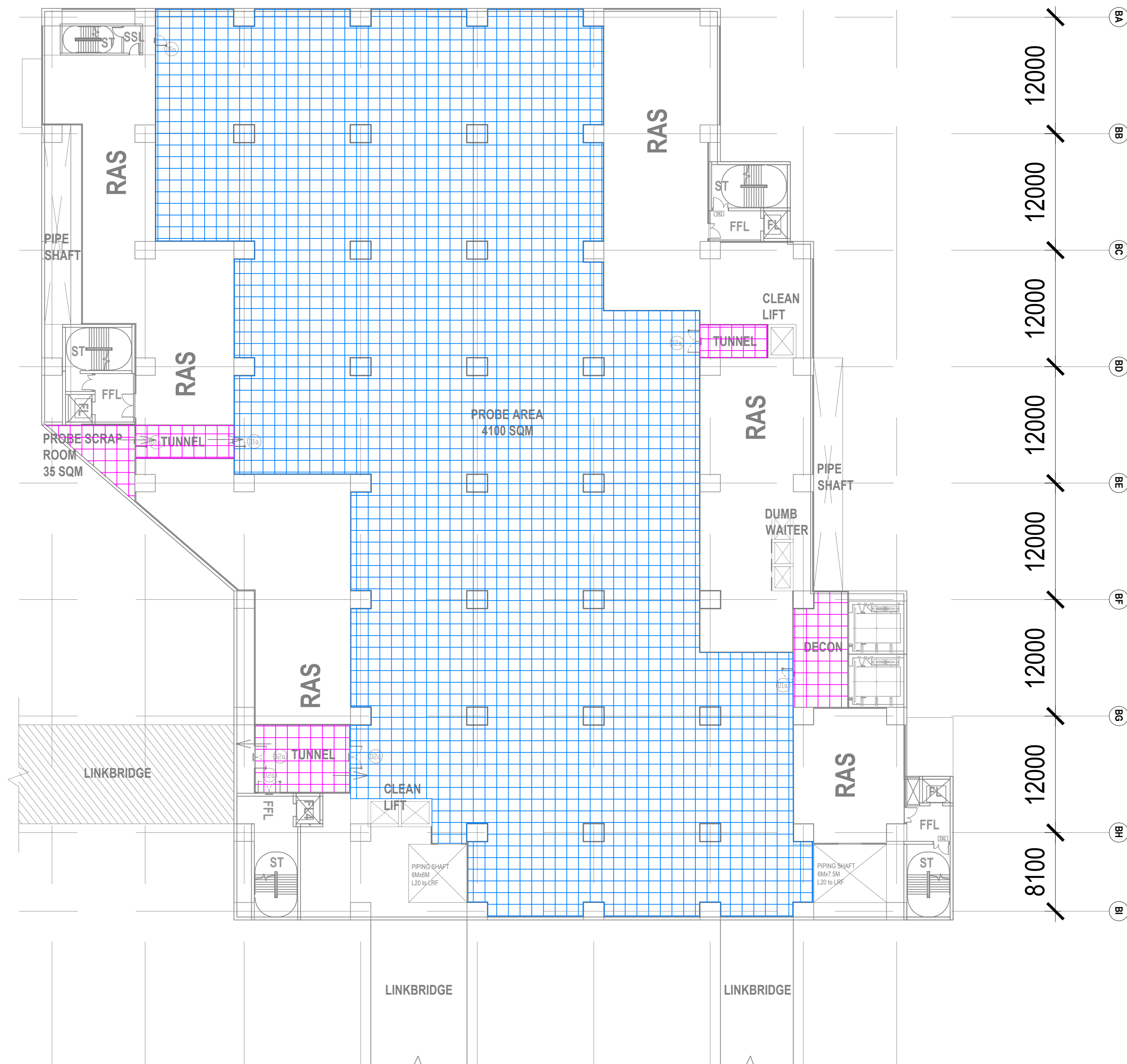
F10E2 L30, L40, L50, L70 ,L80 ,L100 CEILING LAYOUT SCALE 1:300
